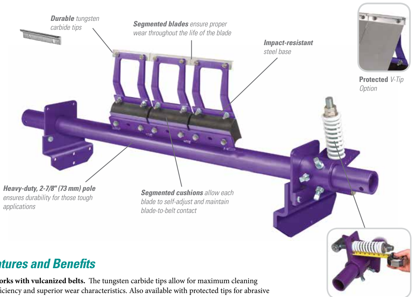
Quick Mount Tensioner (QMT) allows the blade tension to be visually inspected
